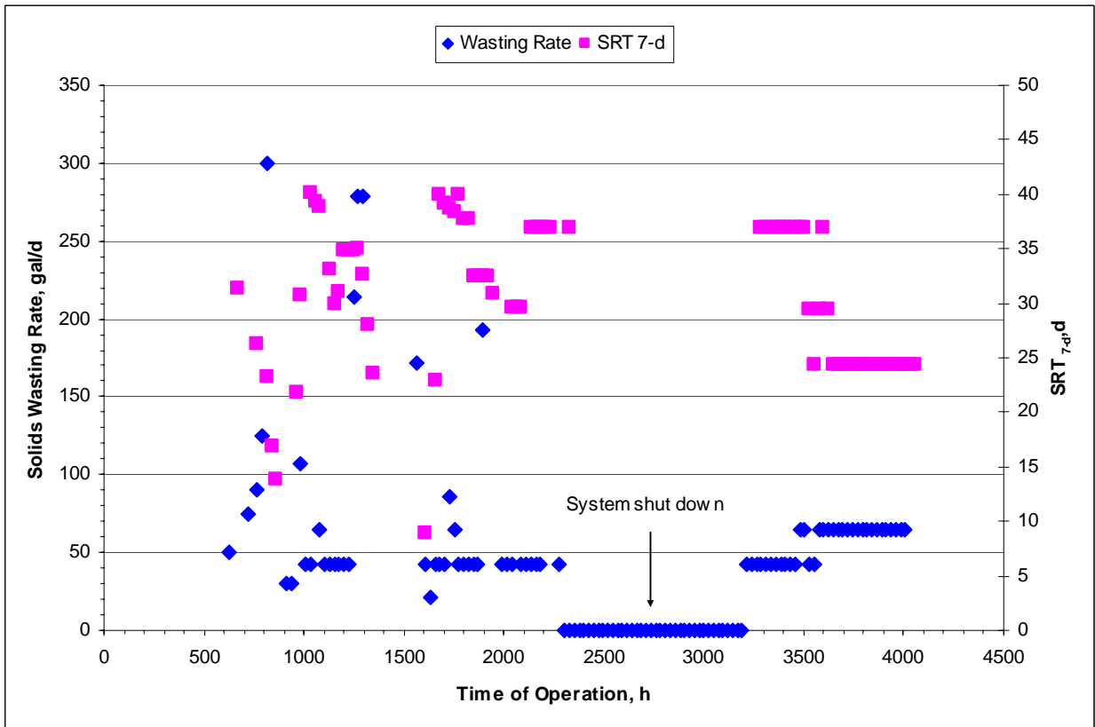
Figure 6-4: HRT and SRT7-d for the Mitsubishi MBR
