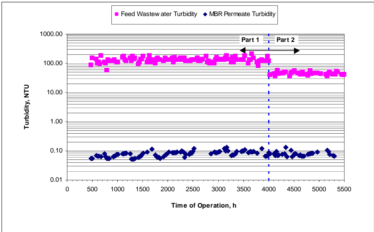
Figure 5-12: Turbidity Removal by the Kubota MBR
