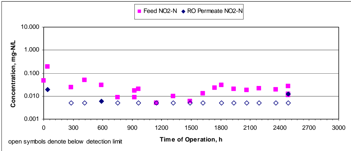
Figure 5-23: Inorganic Nitrogen Removal by the Hydranautics LFC3 RO Membrane
