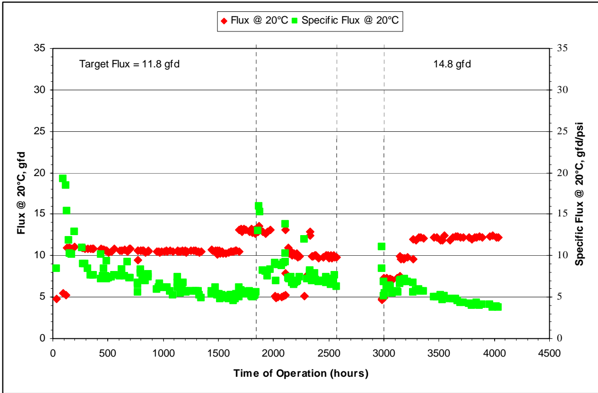
Figure 6-9: Membrane Performance of the Mitsubishi MBR
