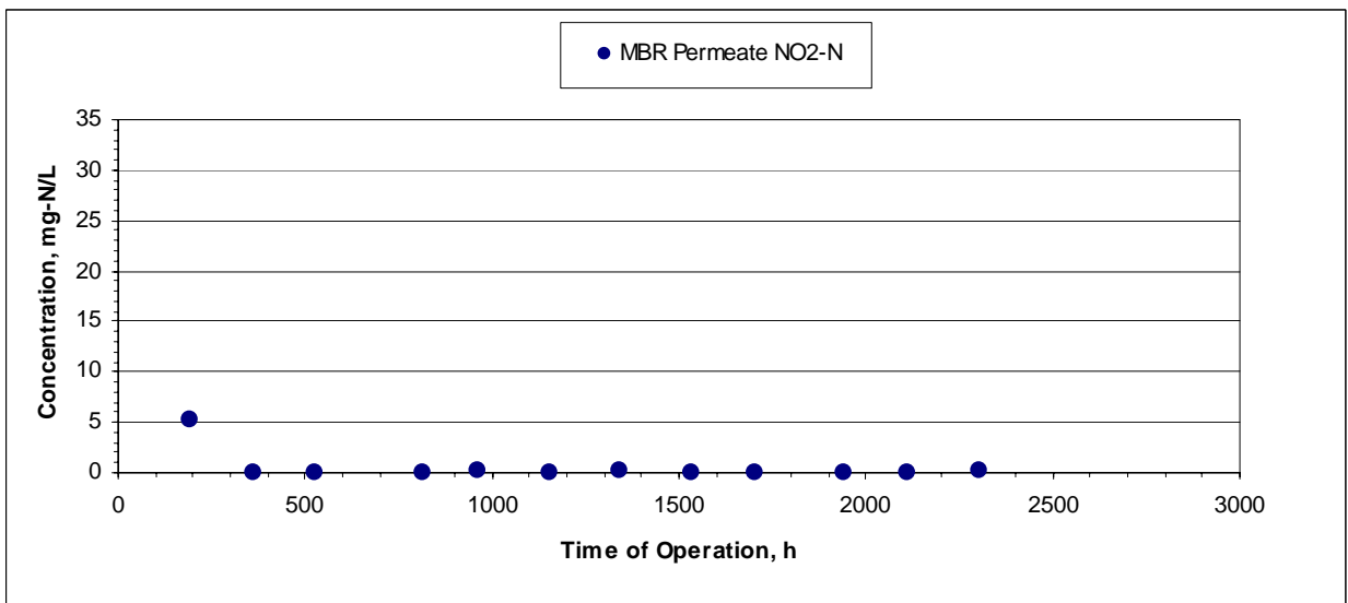
Figure 6-16: Inorganic Nitrogen Species in Mitsubishi MBR
