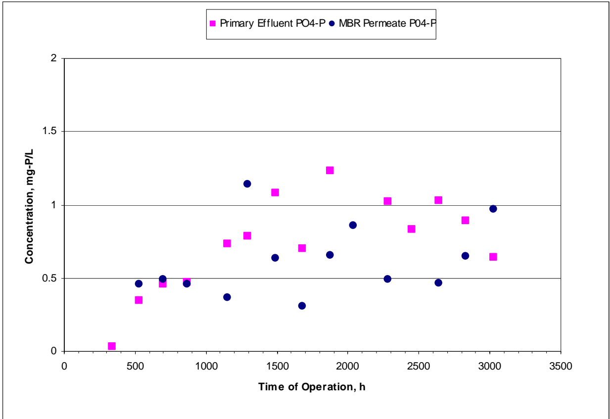
Figure 6-15: Ortho-Phosphate Removal by the Zenon MBR
