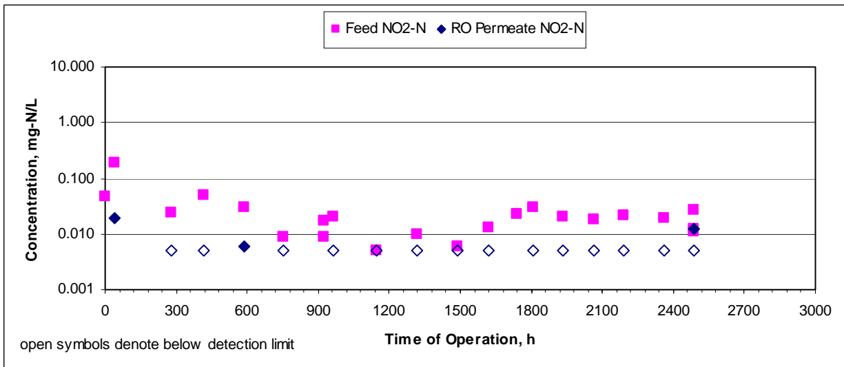
Figure 5-21: Inorganic Nitrogen Removal by the Saehan 4040 BL RO Membrane
