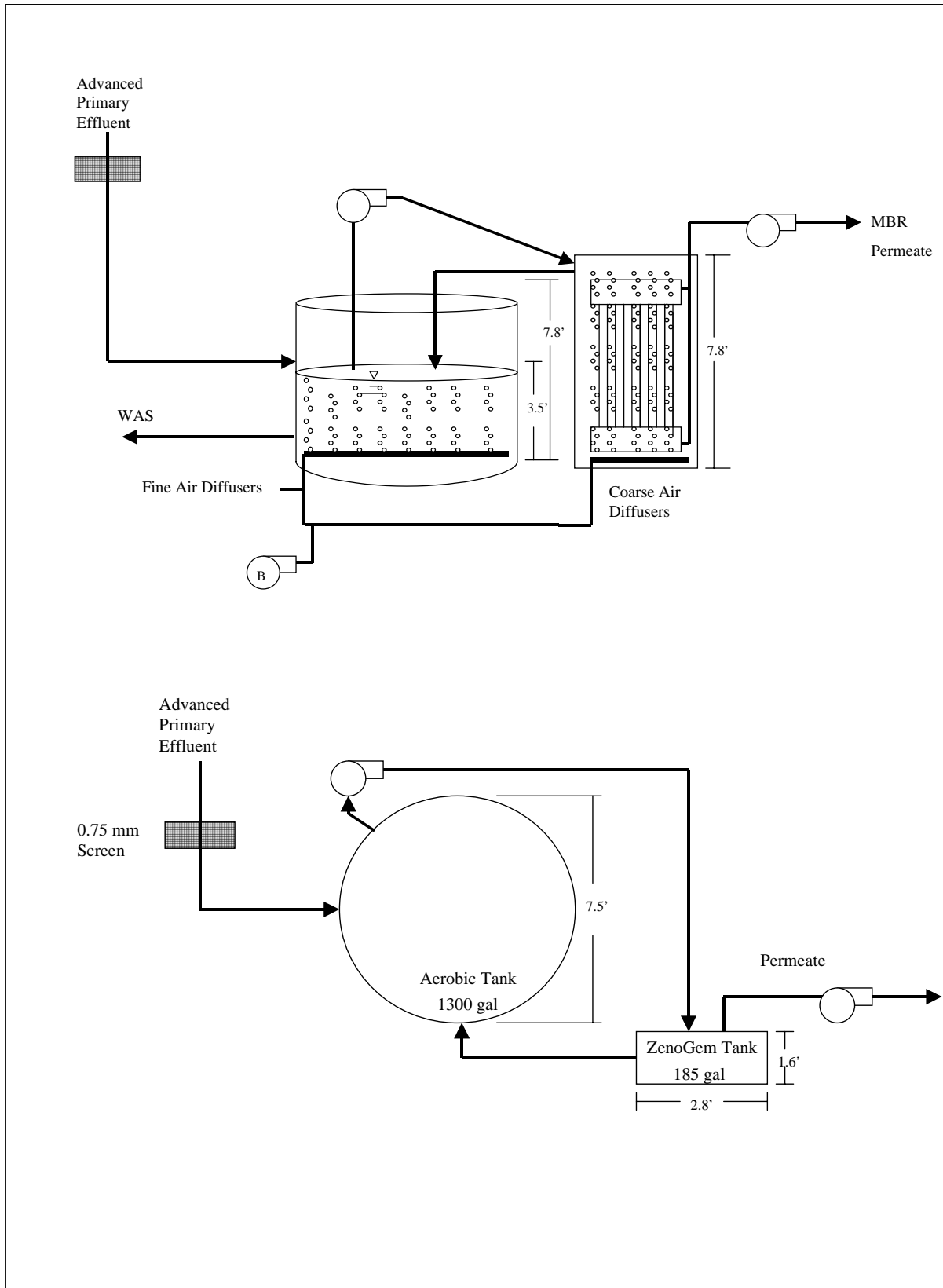
Figure 4-6: Zenon MBR: Side View (Top); Plan View (Bottom)
