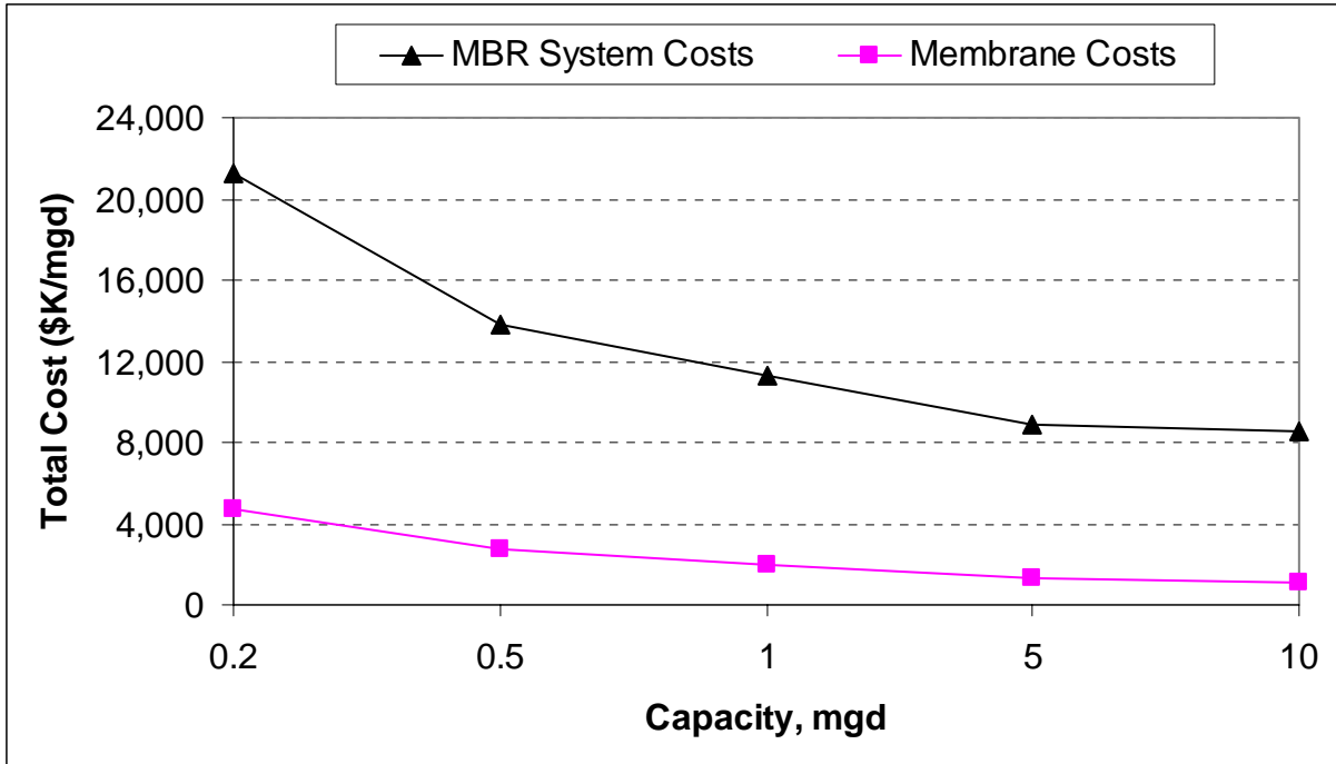
Figure 9-5: Economy of Scale Analysis for MBR Systems Operating on Raw Wastewater
