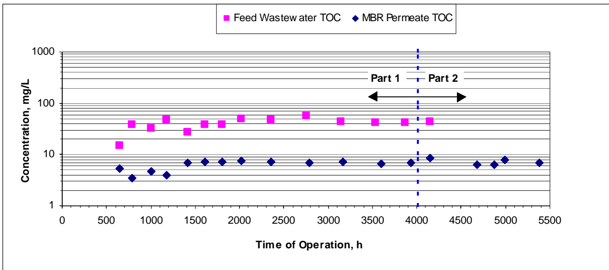
Figure 5-14: Organic Removal by the Kubota MBR
