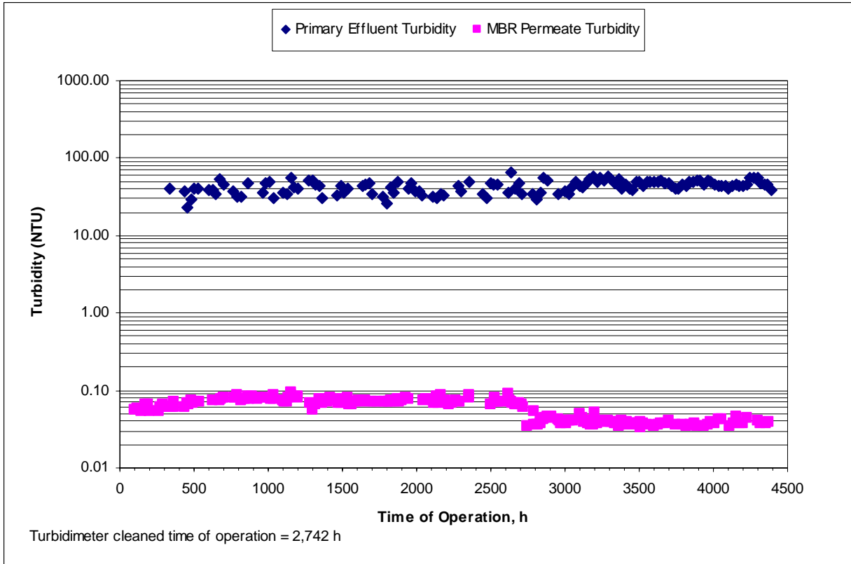
Figure 6-10: Turbidity Removal by the Zenon MBR
