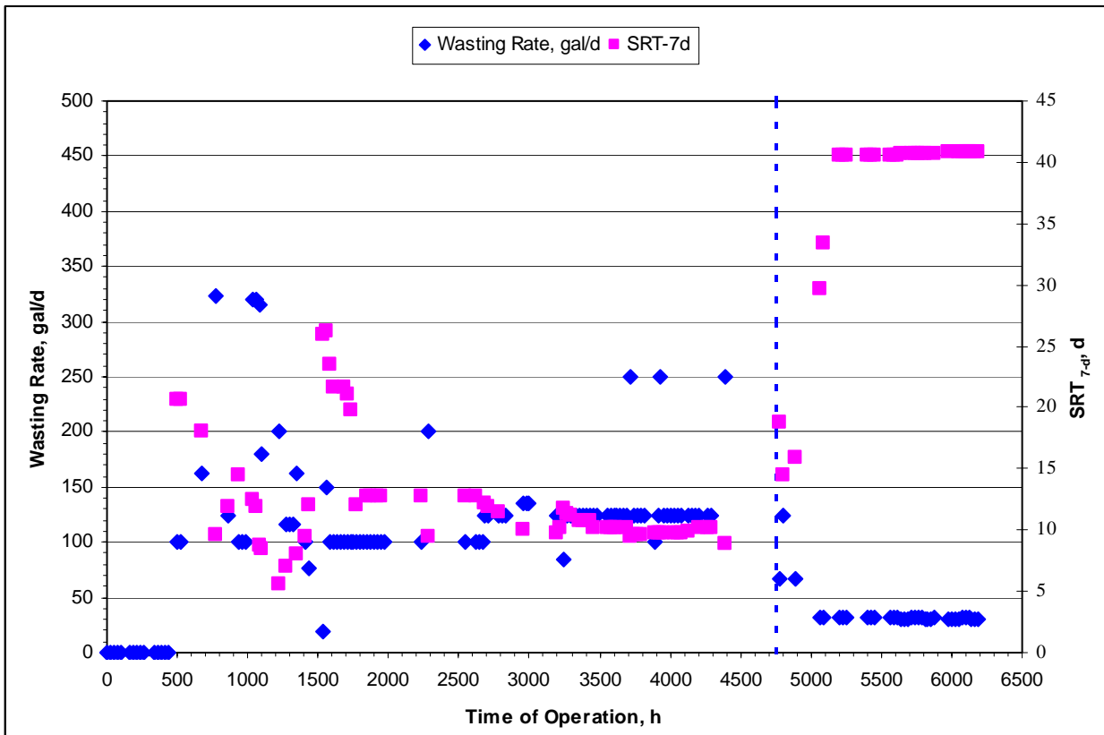
Figure 5-1: HRT and SRT 7-d for the US Filter MBR
