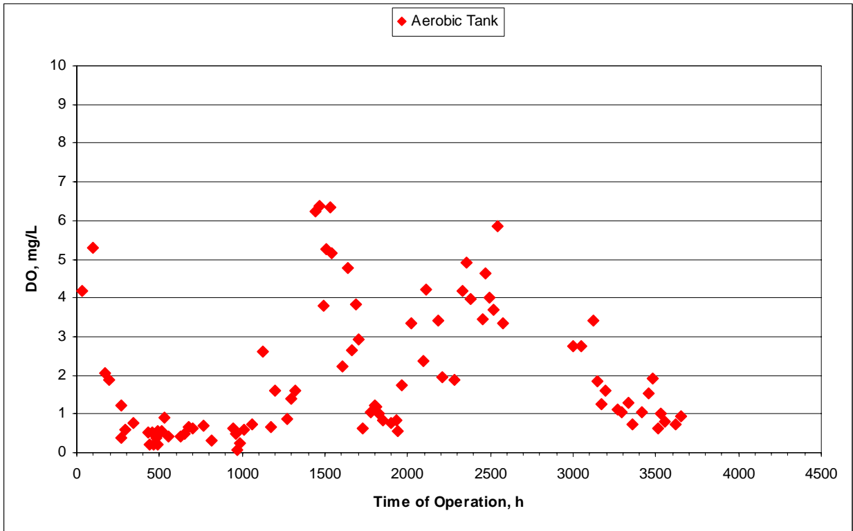
Figure 6-7: DO Concentrations in the Mitsubishi MBR
