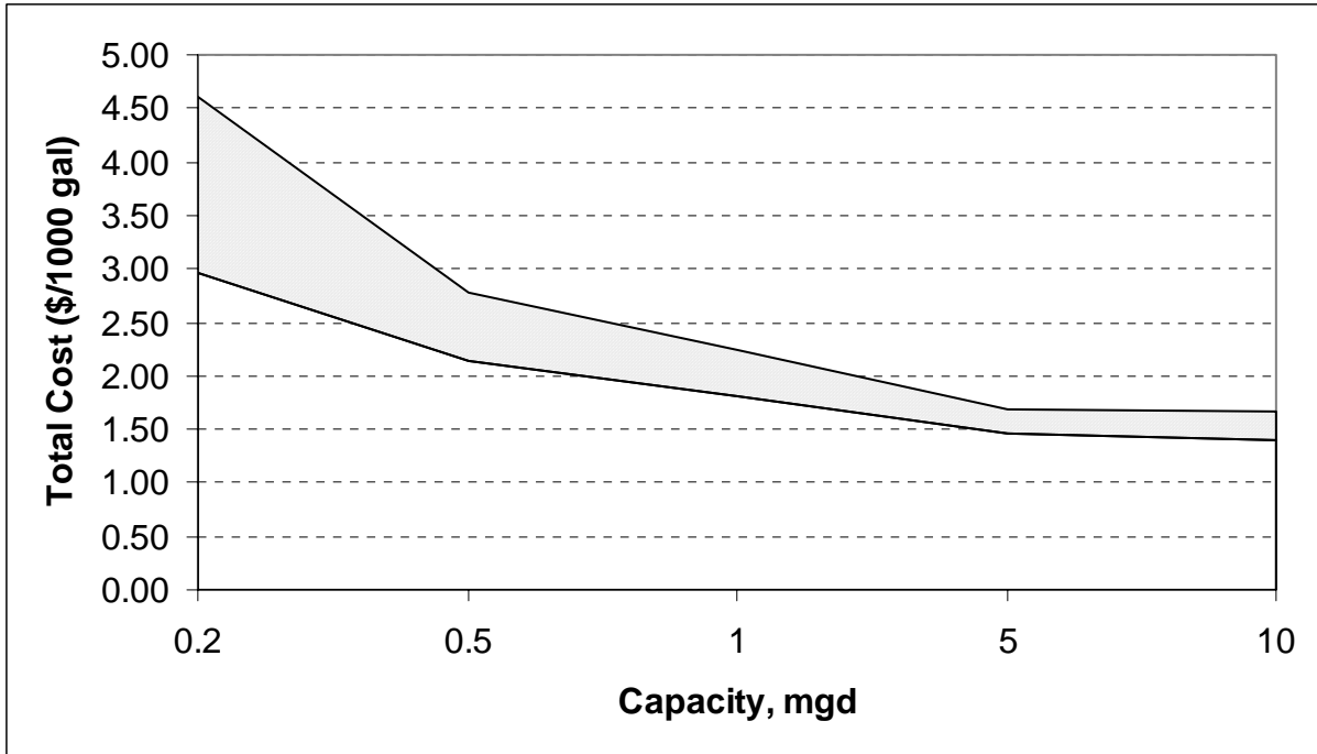
Figure 9-3: Total Costs of Various Capacity MBR Systems Operating on Raw wastewater
