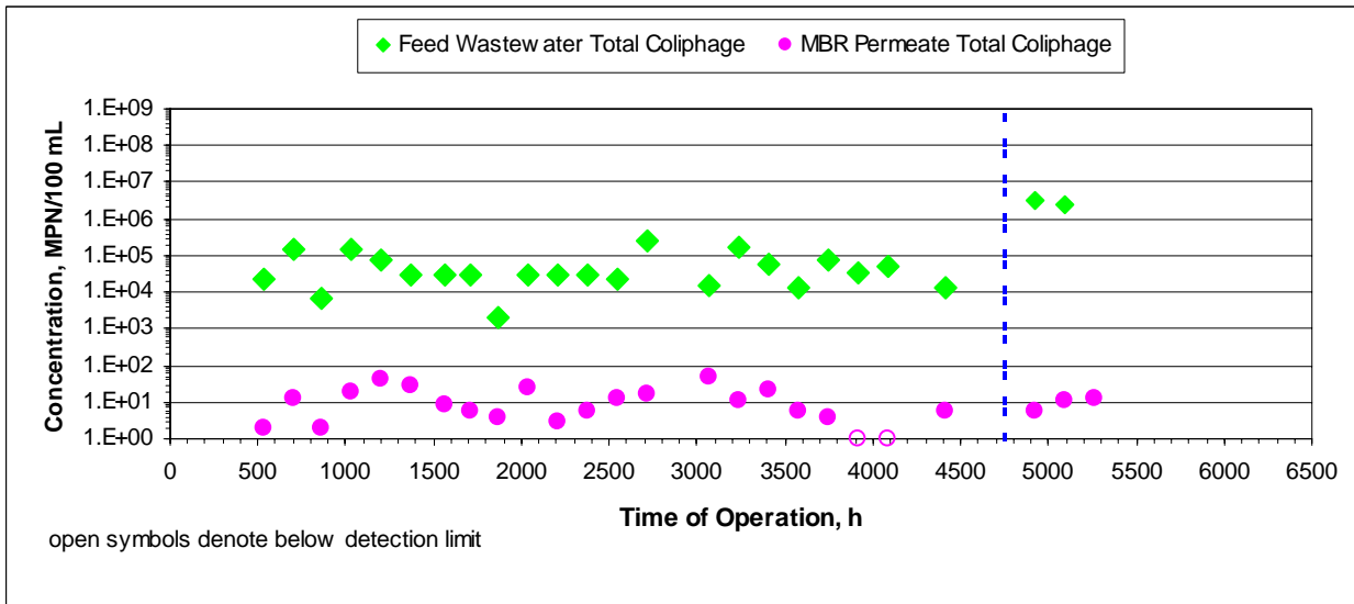
Figure 5-19: Coliform and Coliphage Removal by the US Filter MBR
