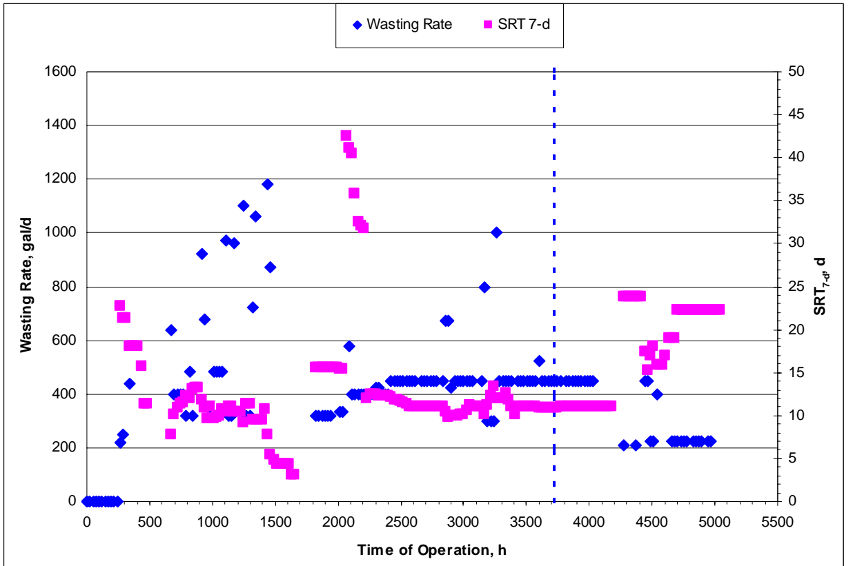
Figure 5-4: HRT and SRT 7-d for the Kubota MBR
