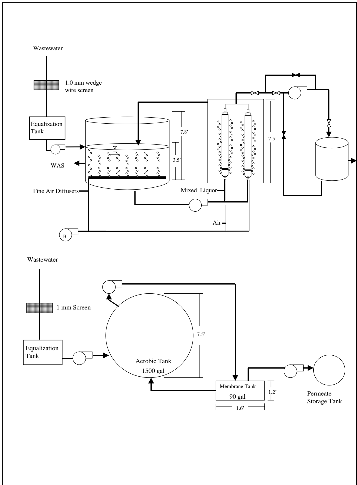
Figure 4-5: US Filter MBR: Side View (Top); Plan View (Bottom)
