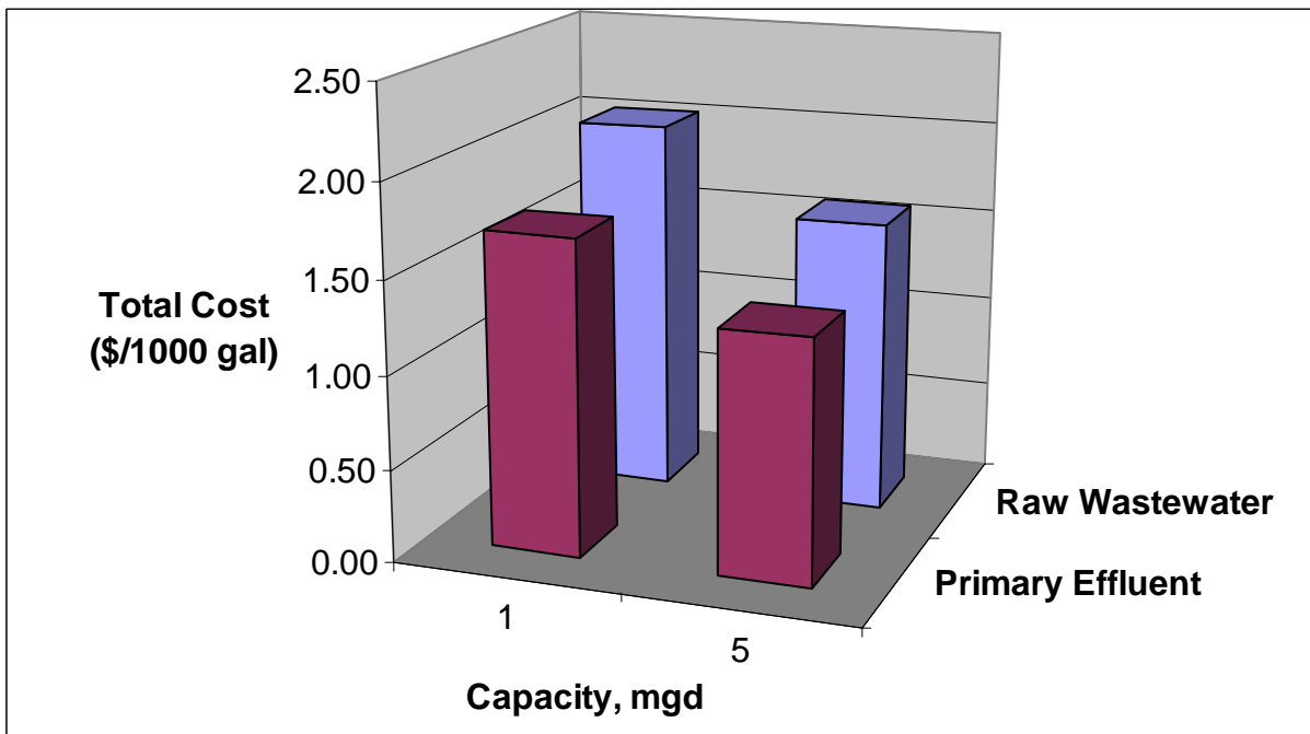
Figure 9-4: Total Costs of 1& 5 MGD MBR Systems (Raw Wastewater / Primary Effluent)
