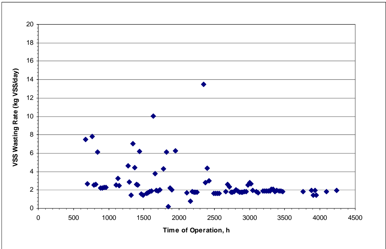
Figure 6-2: Mixed Liquor Solids Concentration for the Zenon MBR
