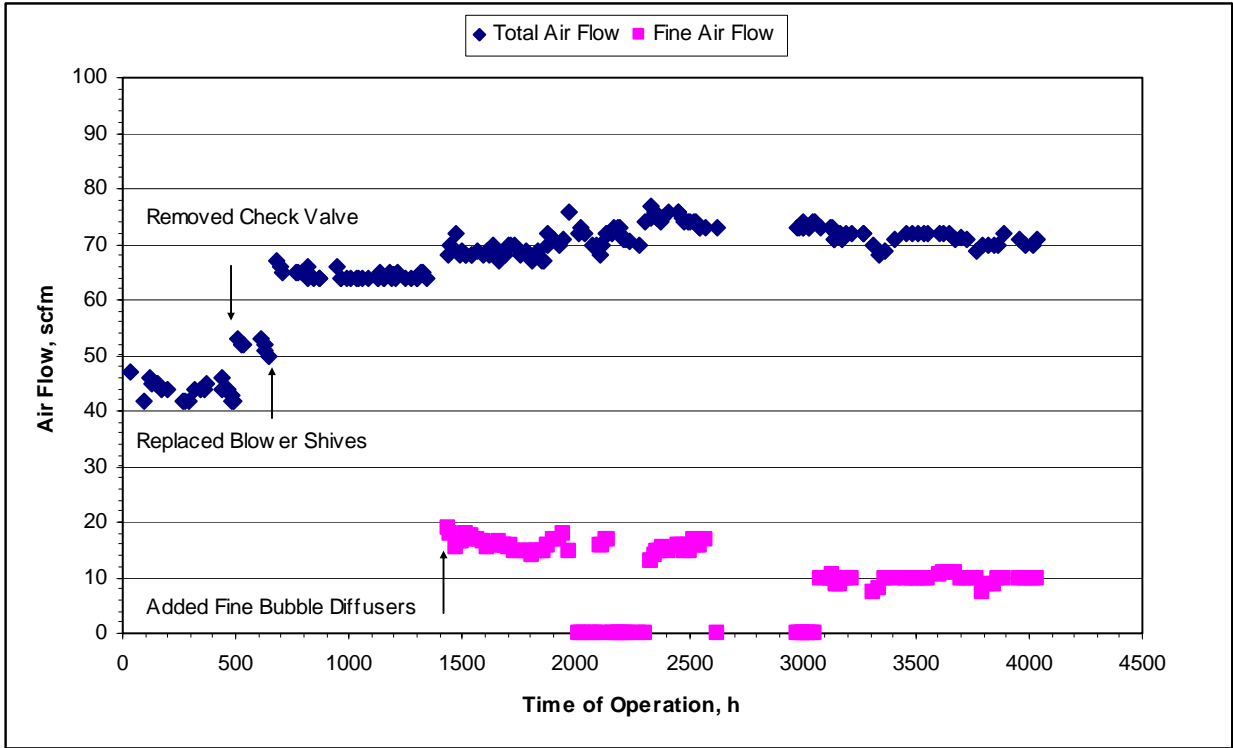
Figure 6-6: Air Flow to the Mitsubishi MBR
