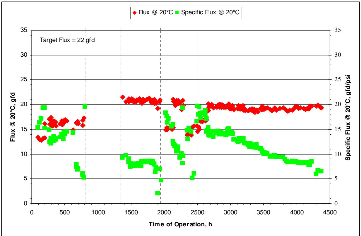
Figure 6-8: Membrane Performance of the Zenon MBR
