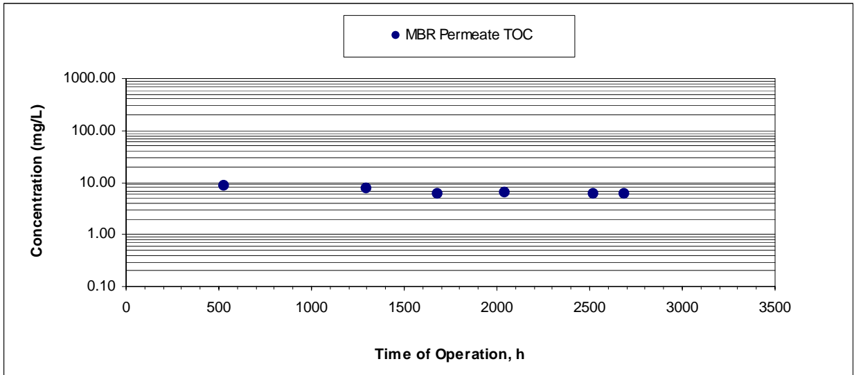
Figure 6-12: Organics Removal by the Zenon MBR
