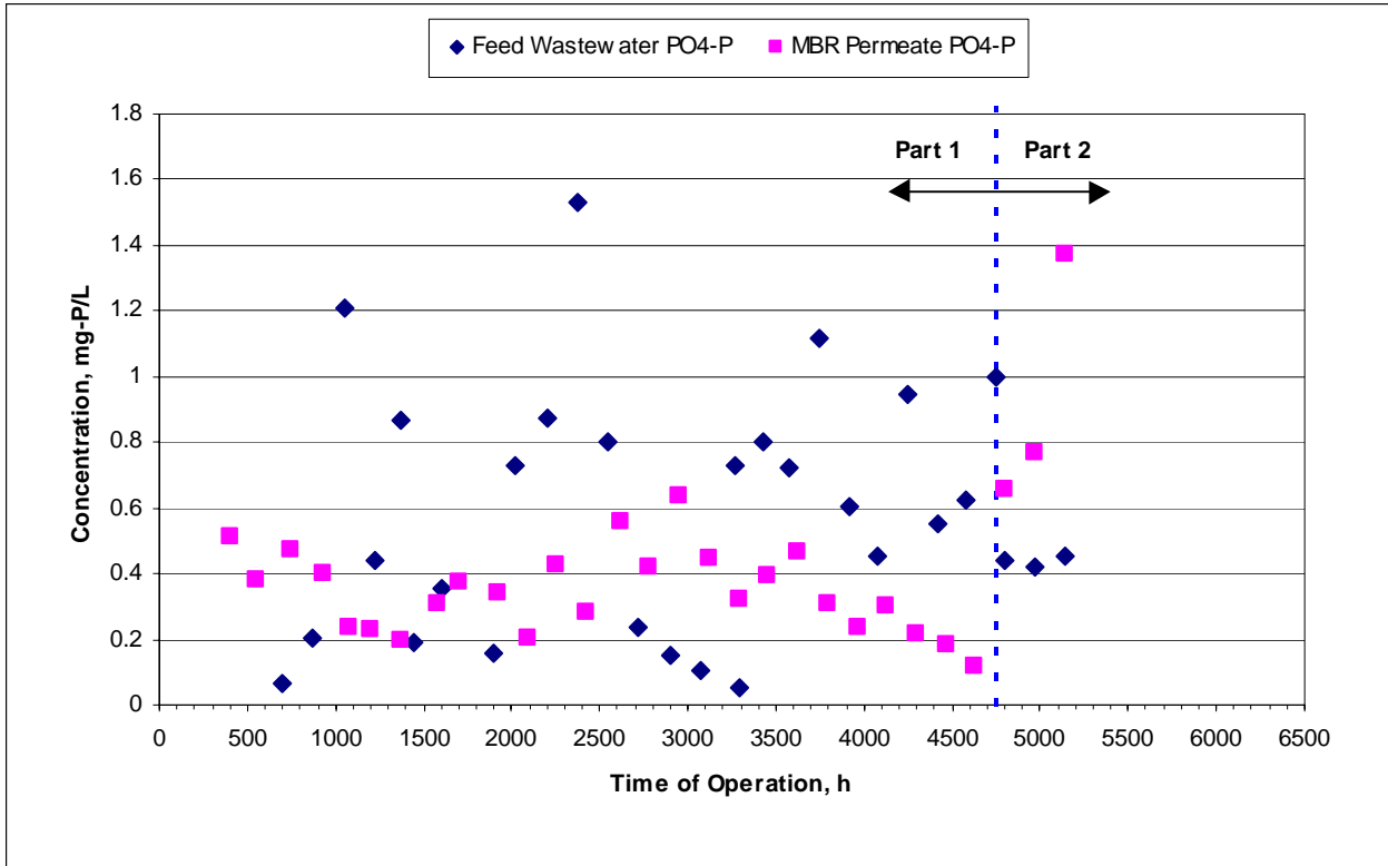
Figure 5-17: Ortho-Phosphate Removal by the US Filter MBR
