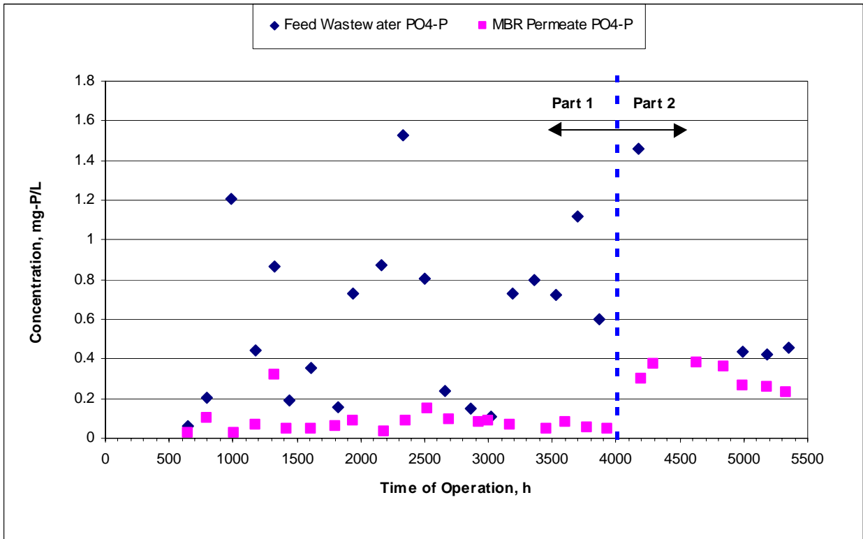
Figure 5-18: Ortho-Phosphate Removal by the Kubota MBR
