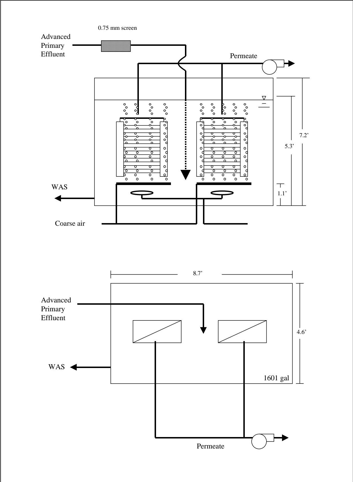
Figure 4-7: Mitsubishi MBR: Side View (Top); Plan View (Bottom)
