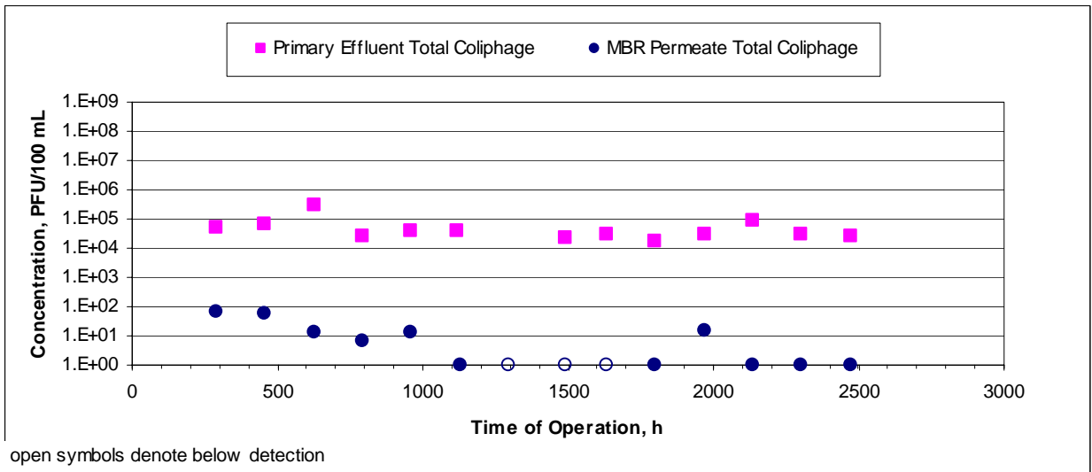
Figure 6-19: Coliform and Coliphage Removal by the Mitsubishi MBR
