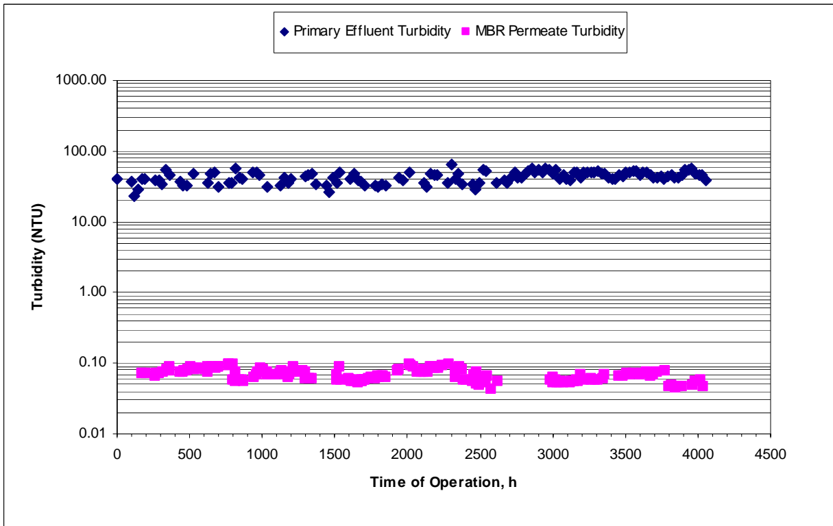
Figure 6-11: Turbidity Removal by the Mitsubishi MBR
