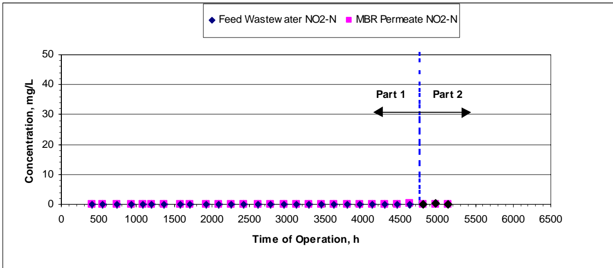
Figure 5-15: Inorganic Nitrogen Removal by the US Filter MBR
