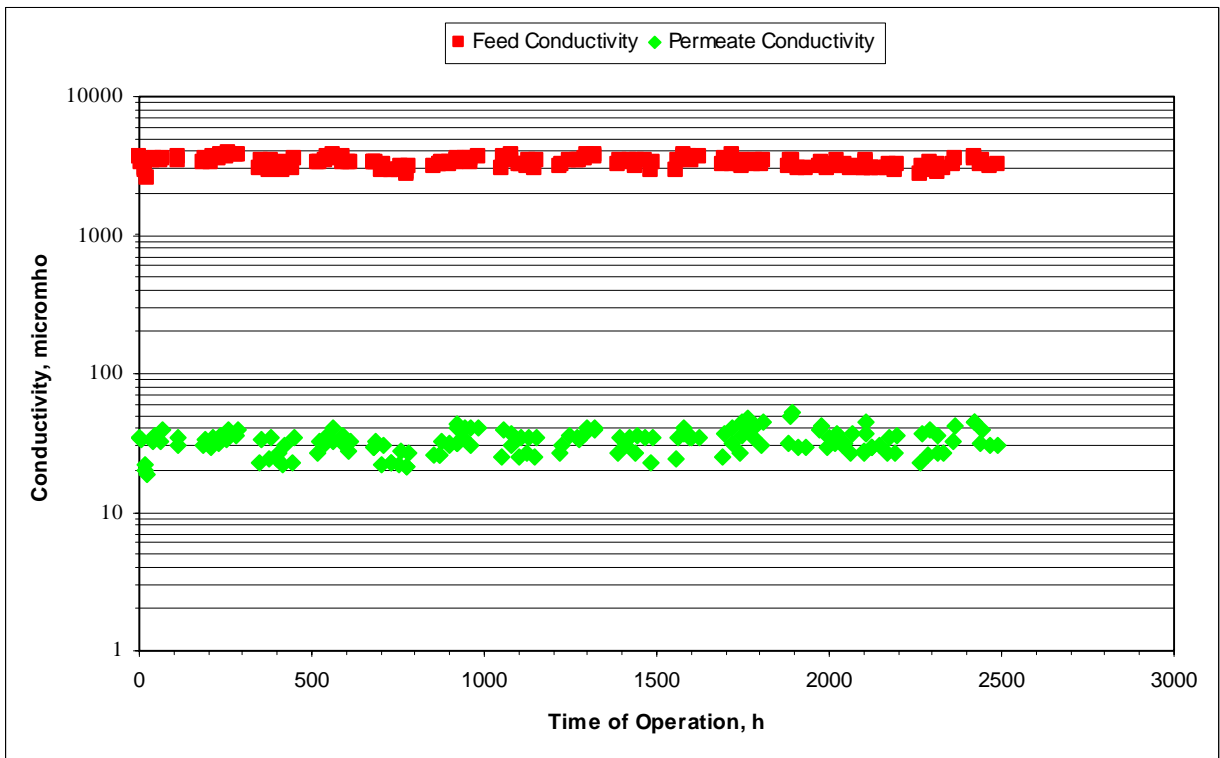
Figure 5-26: Conductivity Profile Across the Hydranautics LFC3 RO Membrane
