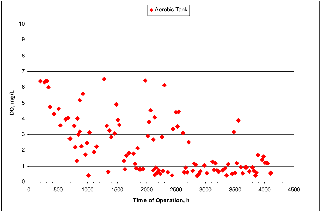
Figure 6-3: DO Concentrations in the Zenon MBR
