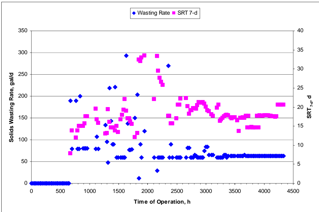
Figure 6-1: HRT and SRT7-d for the Zenon MBR
