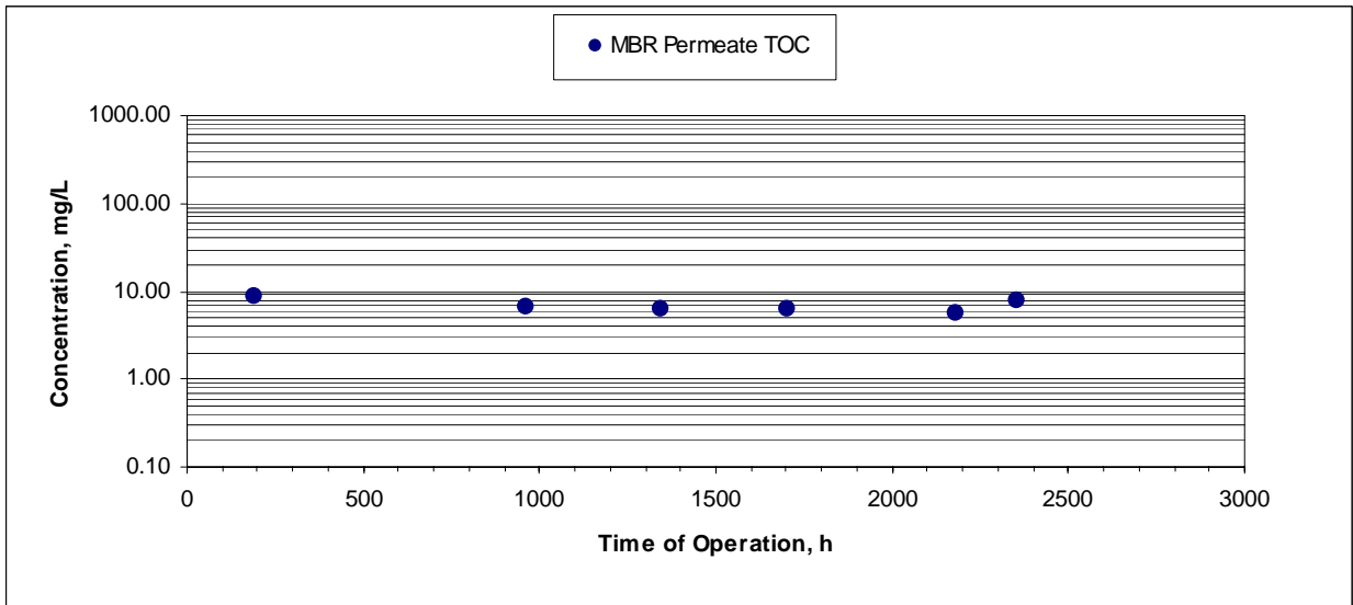
Figure 6-13: Organics Removal by the Mitsubishi MBR
