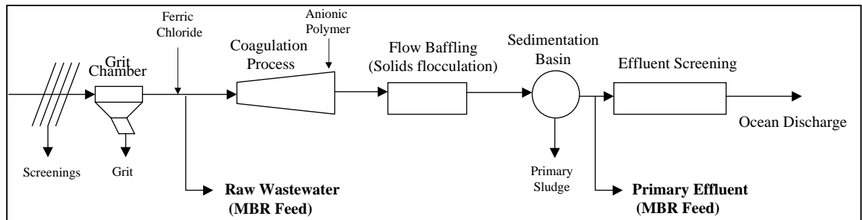
Figure 4-1: Schematic Diagram of the Point Loma Advanced Wastewater Treatment Plant
