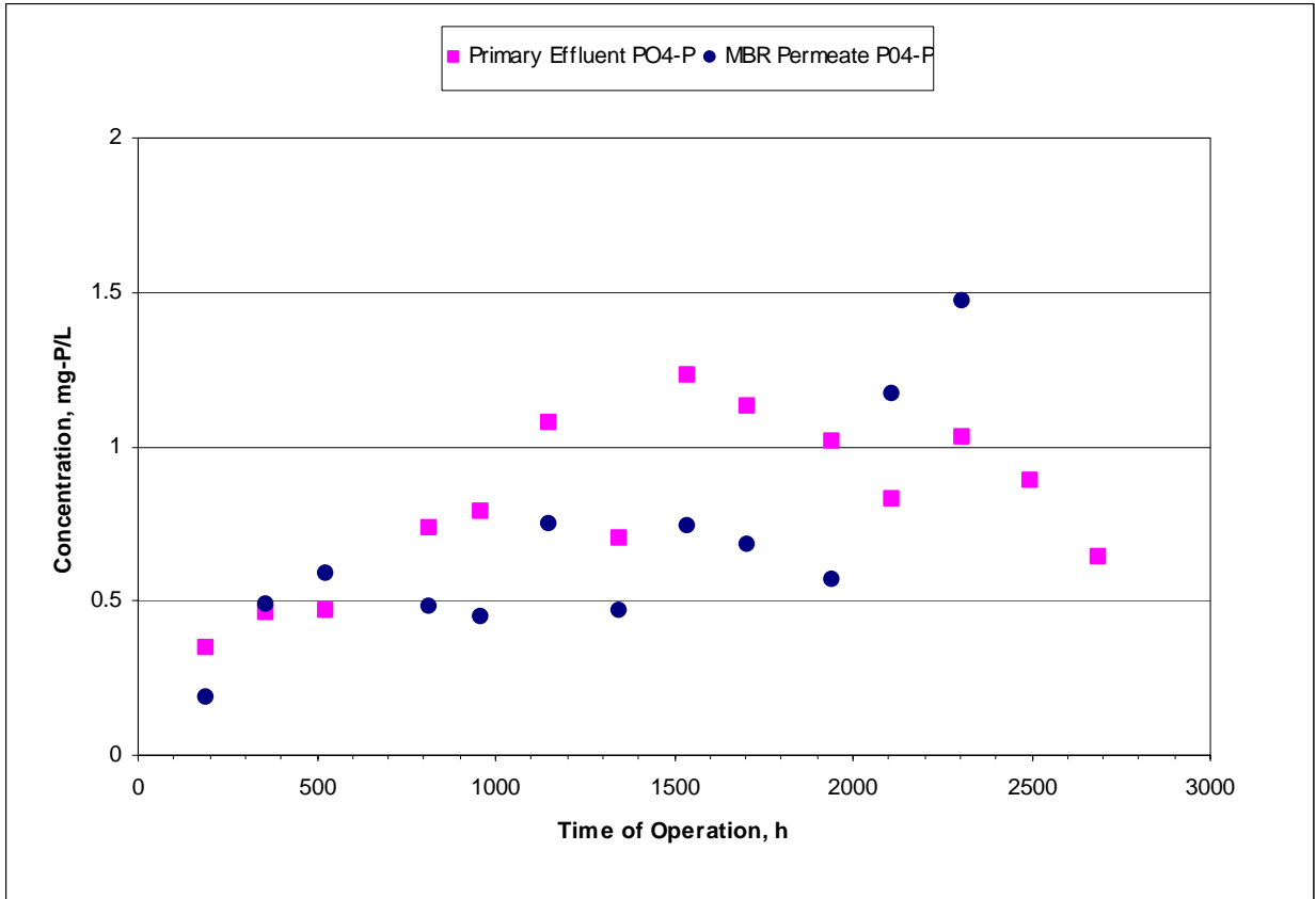
Figure 6-17: Ortho-Phosphate Removal by the Mitsubishi MBR
