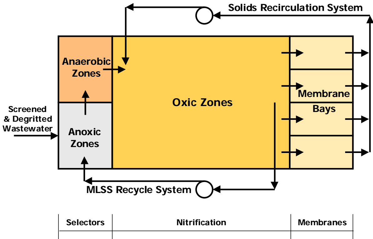
Figure 9-2 MBR Reclaimed Water Schematic: Forward Flow (Top); Recycled Flow (Bottom)
