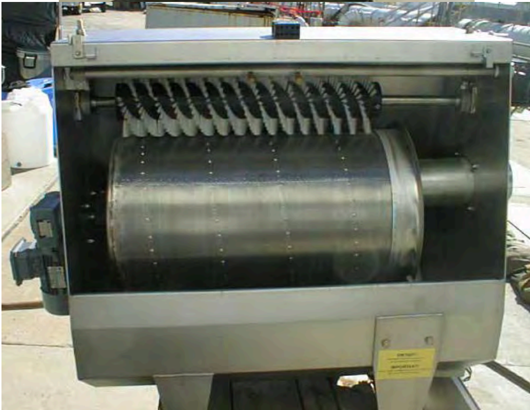
Pre-Screen (Roto-Sieve Model 6013-11)
