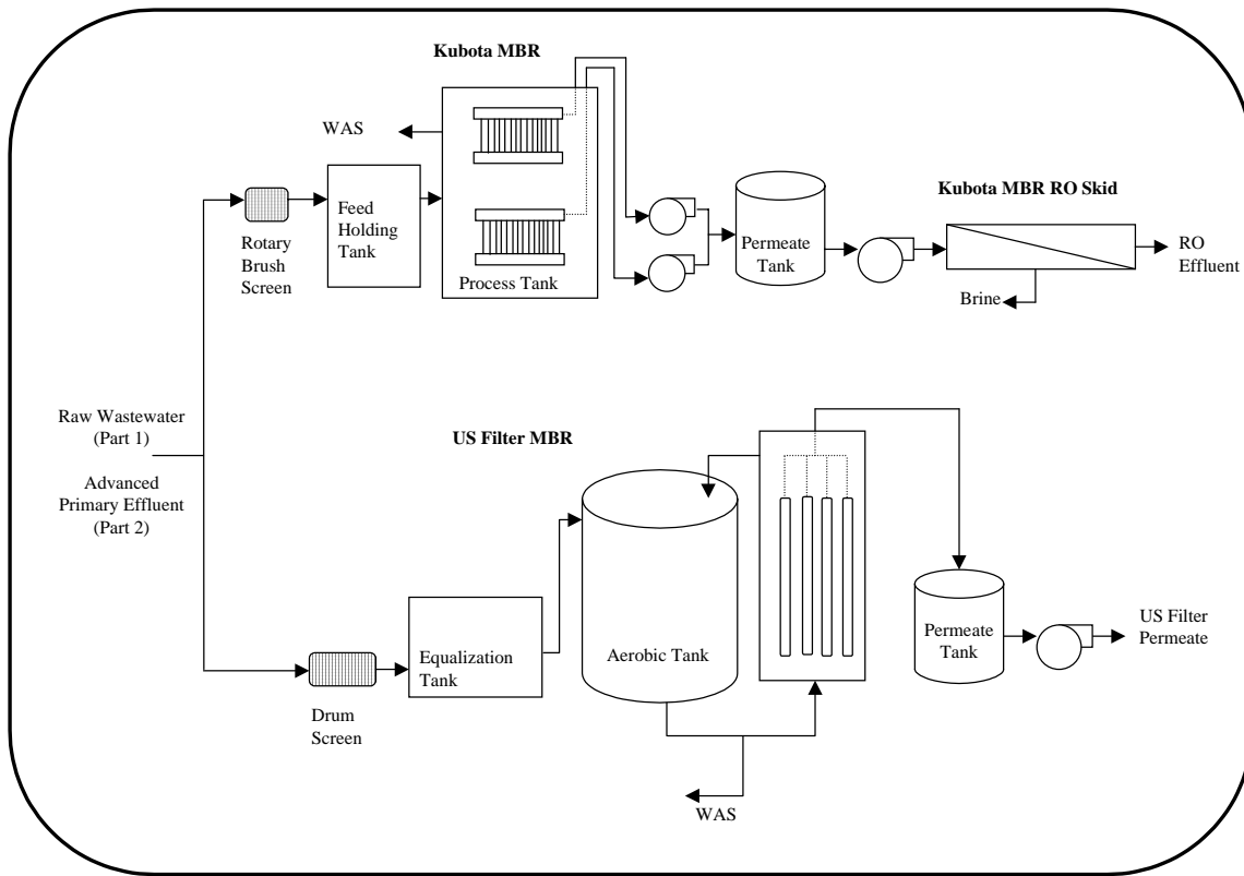
Figure 4-2: Schematic Diagram of Pilot Treatment Train during Phase I (Part 1 & Part 2)
