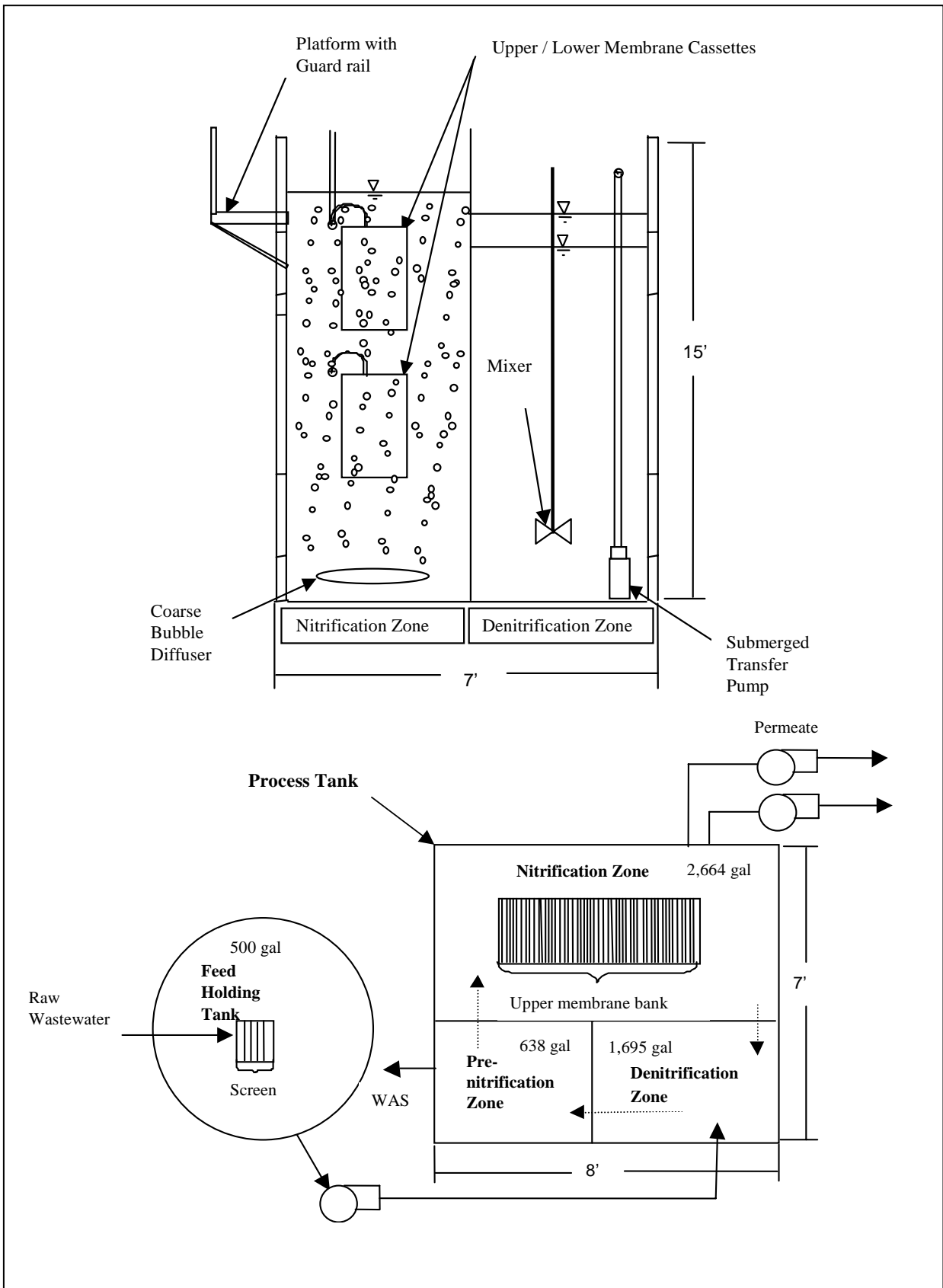
Figure 4-4: Kubota MBR: Side View (Top); Plan View (Bottom)
