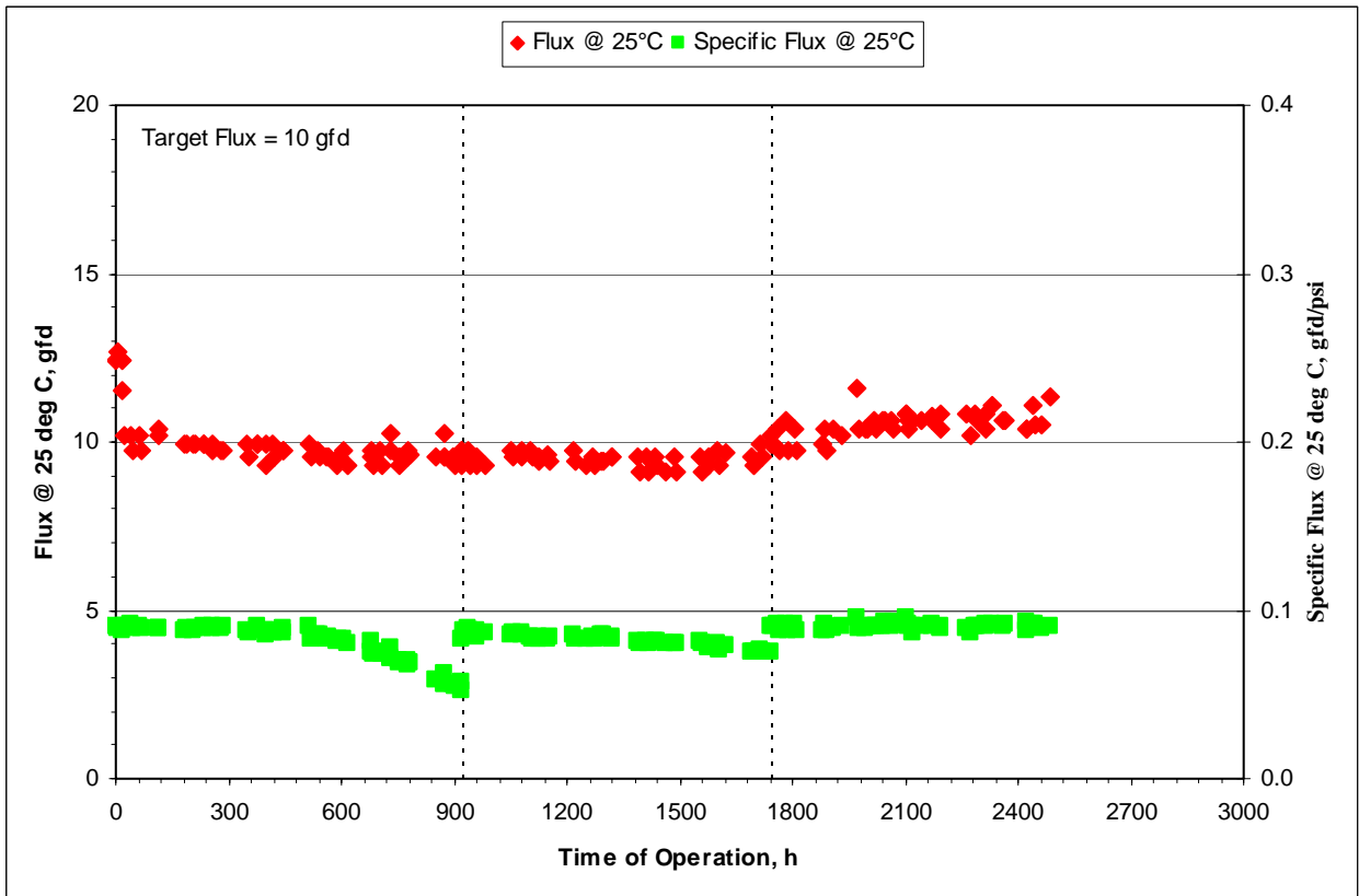
Figure 5-10: Hydranautics LFC3 RO Membrane Performance
