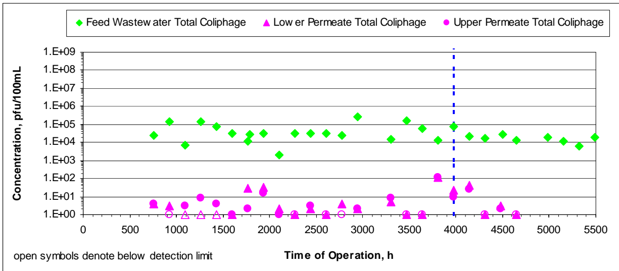
Figure 5-20: Coliform and Coliphage Removal by the Kubota MBR
