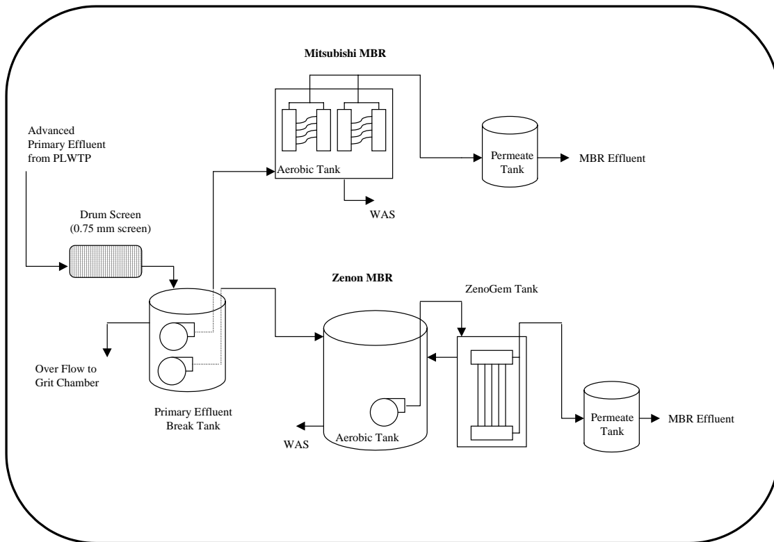
Figure 4-3: Schematic Diagram of Pilot Treatment Train during Phase II
