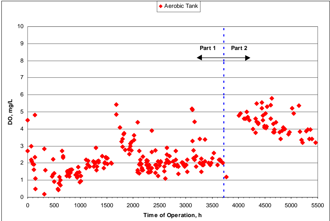
Figure 5-5: DO Concentration in the Kubota MBR
