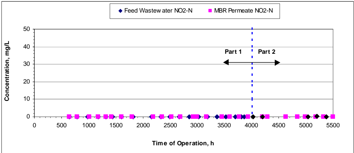
Figure 5-16: Inorganic Nitrogen Removal by the Kubota MBR
