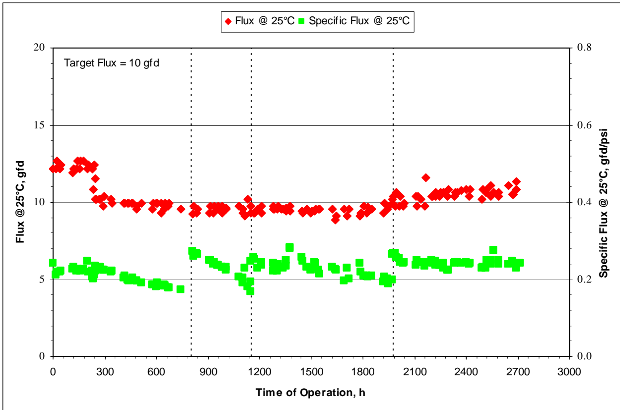
Figure 5-9: Saehan 4040 BL RO Membrane Performance
