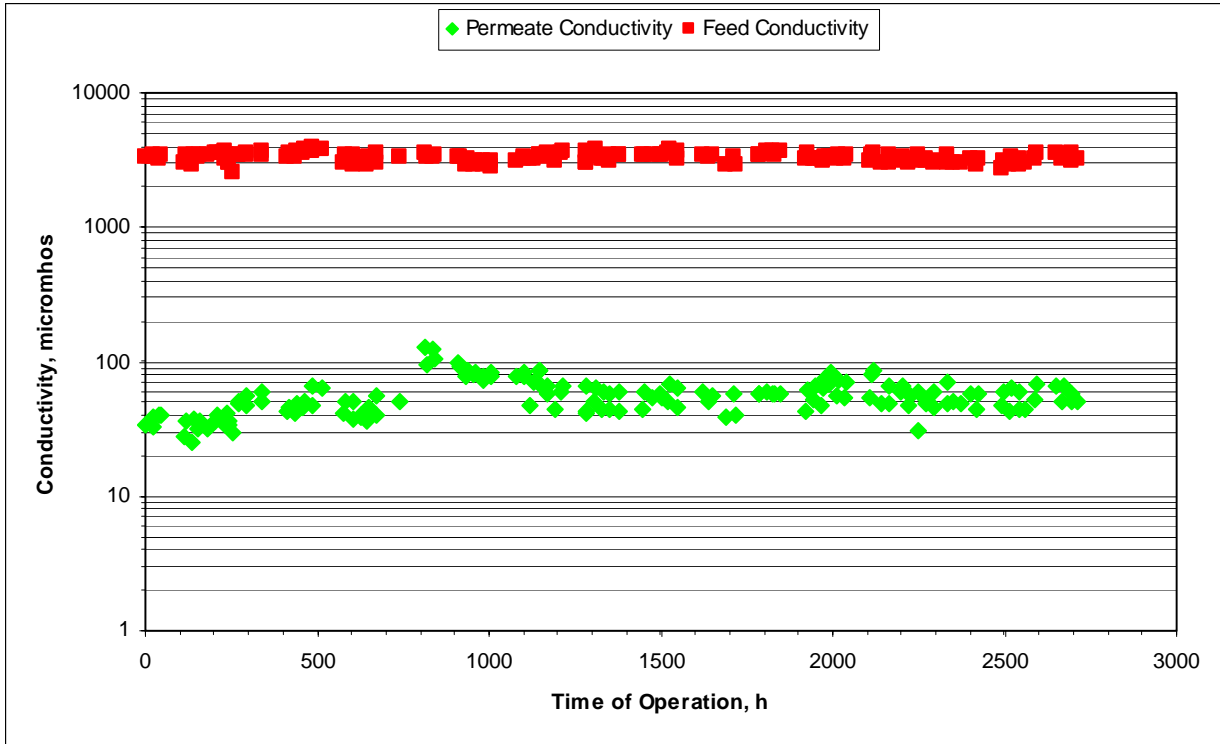
Figure 5-25: Conductivity Profile across the Saehan 4040 BL RO Membrane
