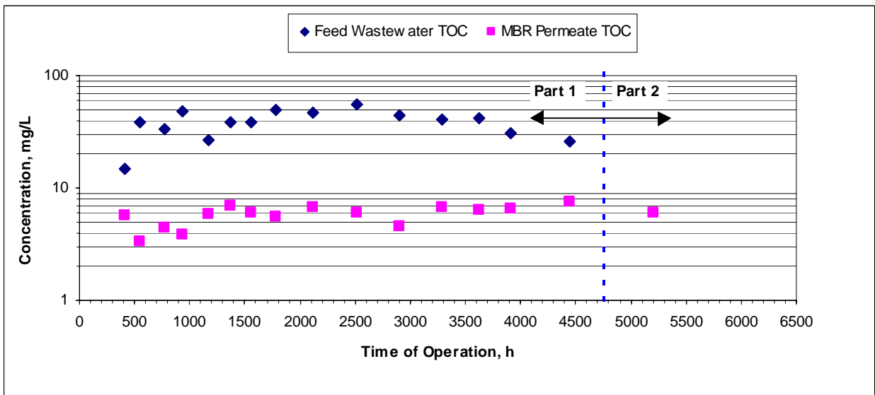
Figure 5-13: Organic Removal by the US Filter MBR
