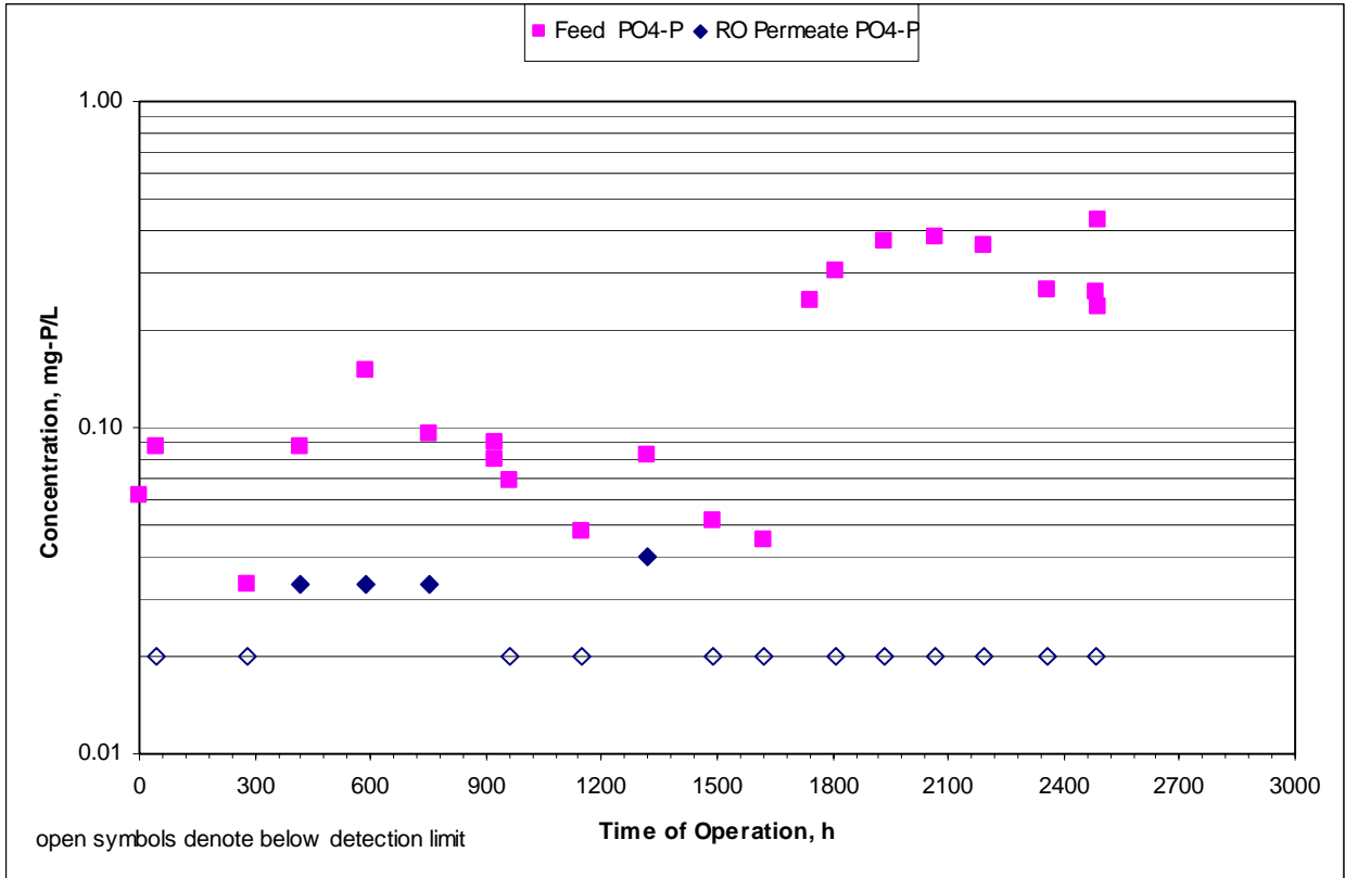
Figure 5-24: Ortho-Phosphate Removal by the Hydranautics LFC3 RO Membrane
