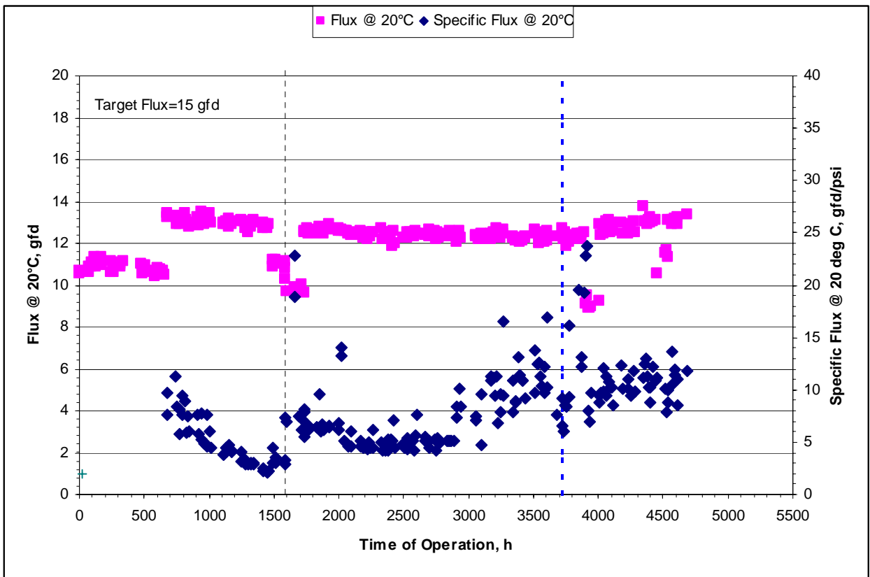
Figure 5-8: Membrane Performance of the Kubota MBR
