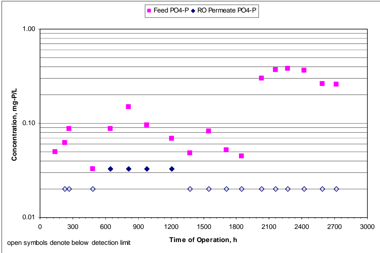
Figure 5-22: Ortho-Phosphate Removal by the Saehan 4040 BL RO Membrane
