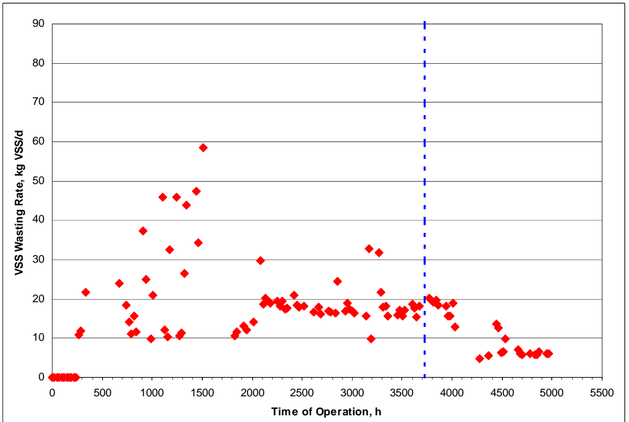
Figure 5-6: Mixed Liquor Solids for the Kubota MBR
