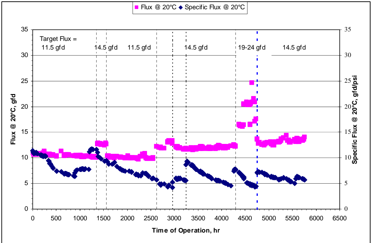
Figure 5-7: Membrane Performance of the US Filter MBR
