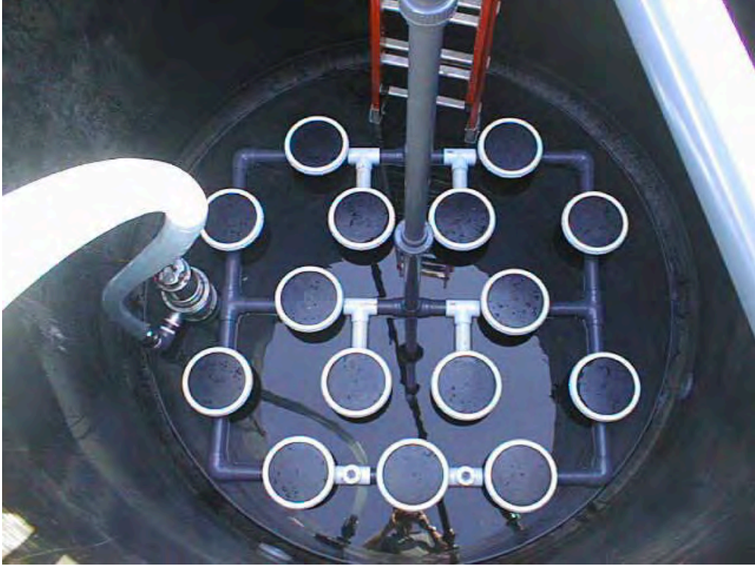
Zenon MBR Aeration Tank with Fine Bubble Diffusers (Plan View)
