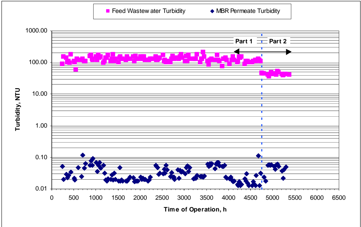
Figure 5-11: Turbidity Removal by the US Filter MBR
