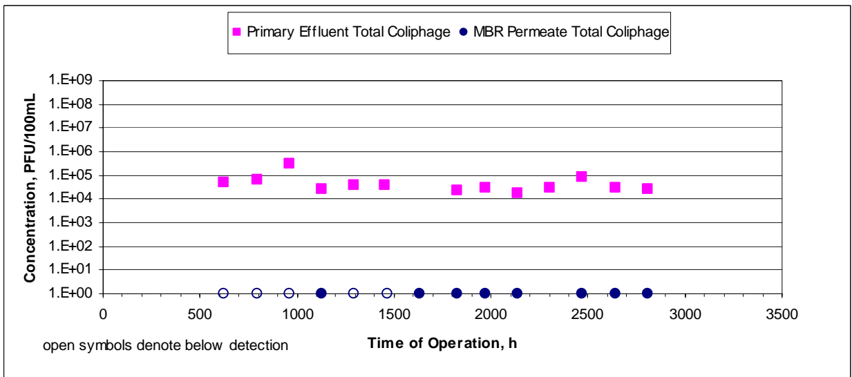
Figure 6-18: Coliform and Coliphage Removal by the Zenon MBR
